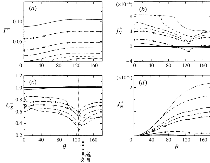
FIGURE 14. Time evolution of the scalar quantities at the interface for Case 4. For caption see figure 6. —, No mass transfer; \cdots\cdots , t^* = 6.5 ; -\cdot-\cdot- , t^* = 15 ; -\cdot-\cdot- , t^* = 35 ; -\cdot-\cdot- , t^* = 75 ; \circ-\circ- , t^* = 125 ; \bullet-\bullet- , t^* = 225 ; —, steady state.
