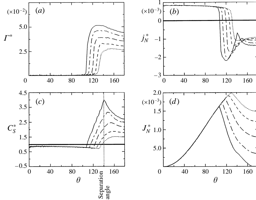
FIGURE 10. Time evolution of the scalar quantities at the interface for Case 3. For caption see figure 6. —, No mass transfer; \cdots , t^* = 5 ; --- , t^* = 9 ; - \cdot - , t^* = 16 ; --- , t^* = 25 ; \rule{0.4pt}{1.2pt} , steady state.
