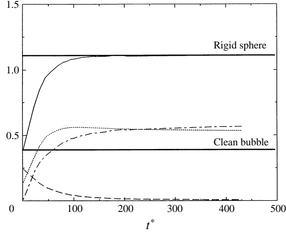
FIGURE 8. Time evolution of the pressure drag coefficient C_p , ( \cdot\cdot\cdot\cdot\cdot ), the normal and tangential viscous drag coefficients C_n ( -\cdot-\cdot- ) and C_t ( -\cdot-\cdot- ), and the total drag coefficient C_D ( — ) for Case 1. Drag coefficients are non-dimensionalized by \frac{1}{2}\pi R^2 \rho U_\infty^2 .
