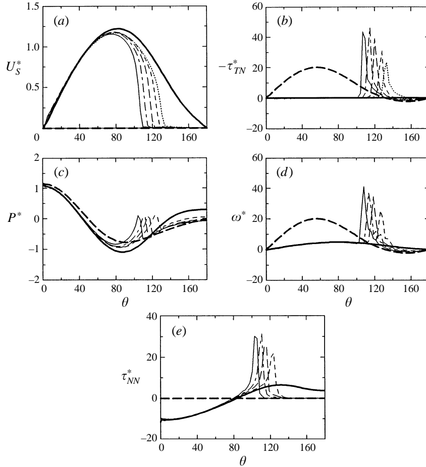
FIGURE 9. Time evolution of the dynamic quantities at the interface for Case 3. For caption see figure 5. —, Clean bubble; — —, rigid sphere; ·····, t^* = 5 ; - · - ·, t^* = 9 ; —, t^* = 16 ; - - - -, t^* = 25 ; —, steady state.
