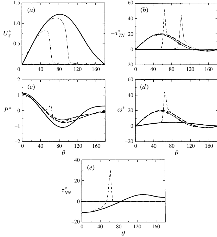
FIGURE 13. Time evolution of the dynamic quantities at the interface for Case 4. For caption see figure 5. —, Clean bubble; — —, rigid sphere; ·····, t^* = 6.5 ; - · - ·, t^* = 15 ; —, steady state.
