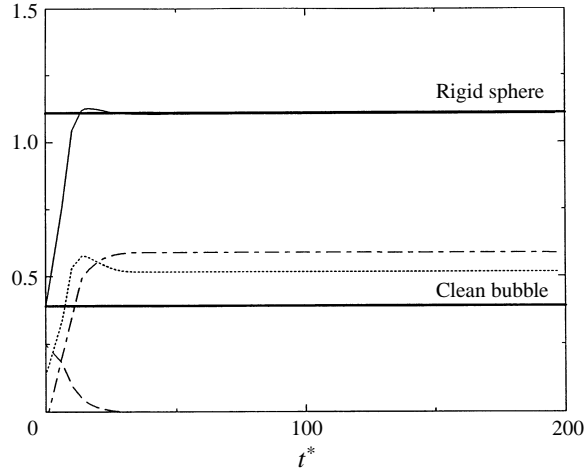
FIGURE 16. Time evolution of the drag coefficients for Case 4: \cdots , C_p ; --- , C_n ; - \cdot - , C_v ; — , C_D .
