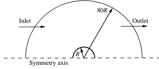
FIGURE 3. Computational domain.
